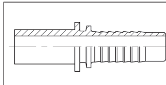
4226 Standpipe straight SP PRODUCT GROUP 300
