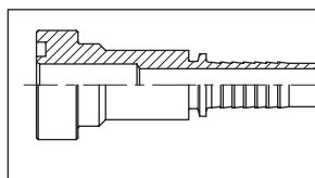
4253 Straight SAE J518 flange Code 62 PRODUCT GROUP 300
