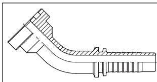
4248 45° SAE J518 flange Code 61 Flange size 5/8" komatsu PRODUCT GROUP 300
