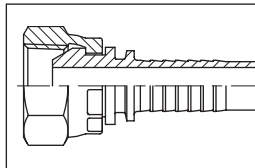
4217~7 JIC short Unified-threaded 45° compact female 74° cone sealing PRODUCT GROUP 300
