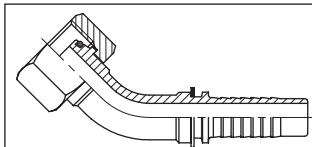
4272~2 Metric 45° bend female 24° cone sealing with O-ring PRODUCT GROUP 300
