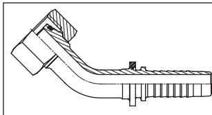
4275~2 Metric 45° bend female 24° cone sealing with O-ring PRODUCT GROUP 300
