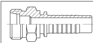
4221 French GAZ Metric GAZ straight male 24° cone, connection for inch pipe PRODUCT GROUP 300
