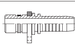
4221 French GAZ Metric GAZ straight male 24° cone, connection for inch pipe PRODUCT GROUP 300
