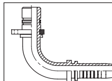
4374 Handle fitting High pressure washer PRODUCT GROUP 300
