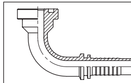
4244~6 90° SAE J518 flange Code 61 Short brazed PRODUCT GROUP 300
