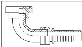
4244~6 90° SAE J518 flange Code 61 Short brazed PRODUCT GROUP 300
