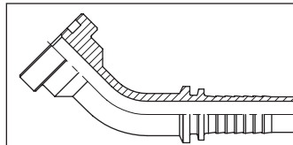
4258 45° SAE J518 flange Code 62 PRODUCT GROUP 300
