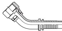
4217 JIC Unified-threaded 45° bend female, 74° cone sealing PRODUCT GROUP 300
